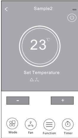
Control form1
